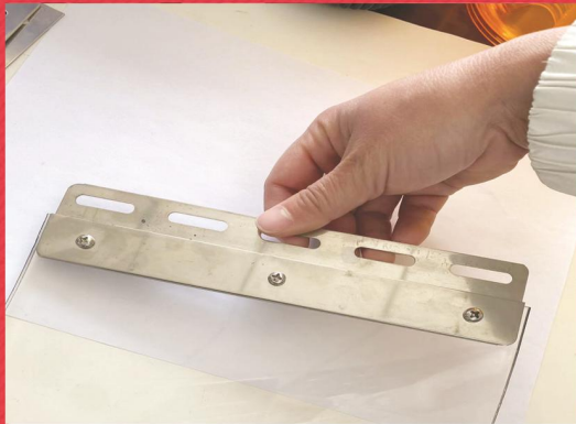
① Fix the clip in the hole of the curtain
